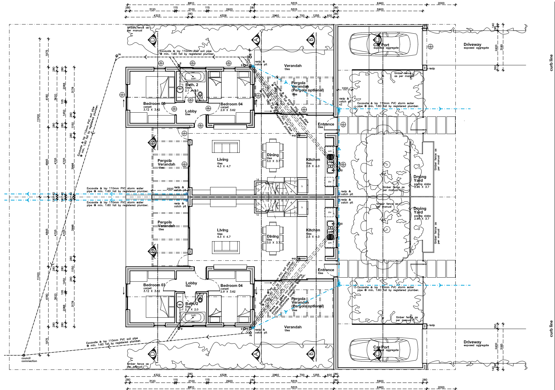
1:100 GROUND FLOOR PLAN
